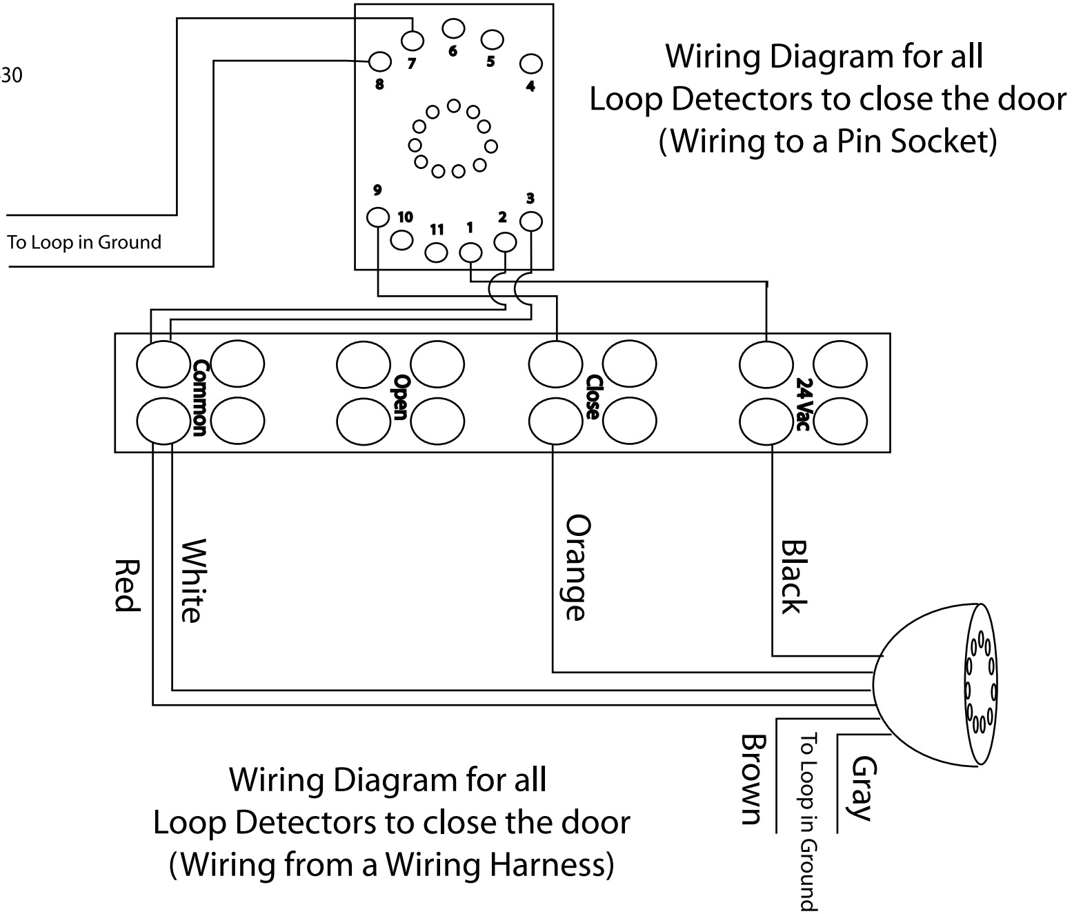
D-TEK Loop Detector (Rear)
