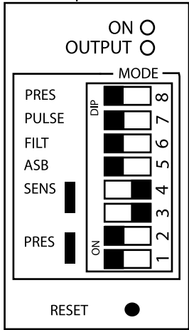
McGANN Loop Detector
