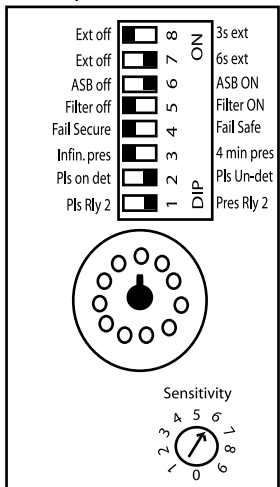
D-TEK Loop Detector (Rear)
